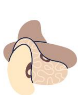
Seed
