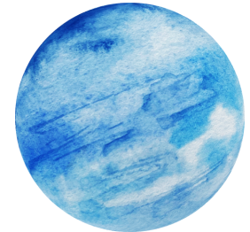
Neptune
